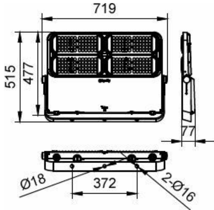
BVP565 LED672/750 430W EP SWB
