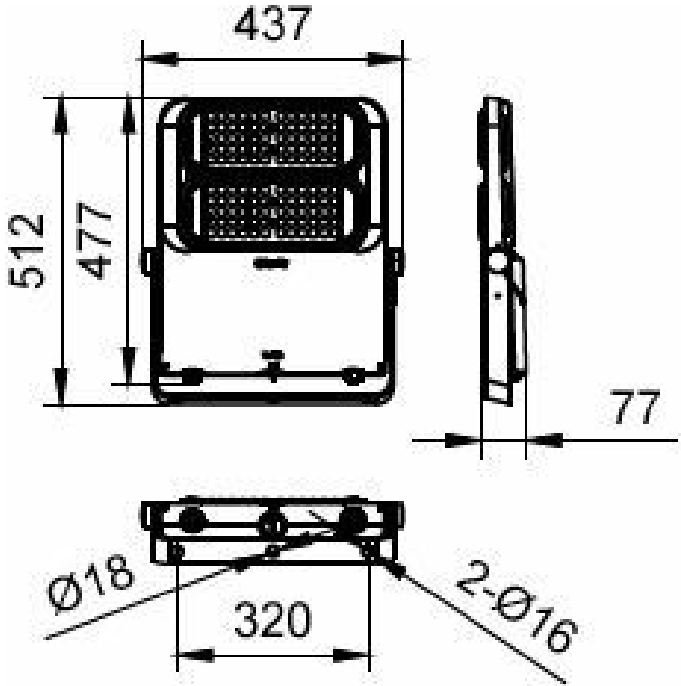
BVP563 LED336/740 220W EP SWB
