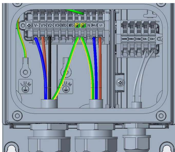
Wiring Diagram
