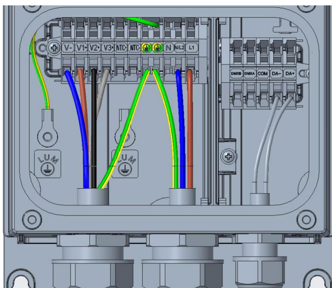
Wiring Diagram
